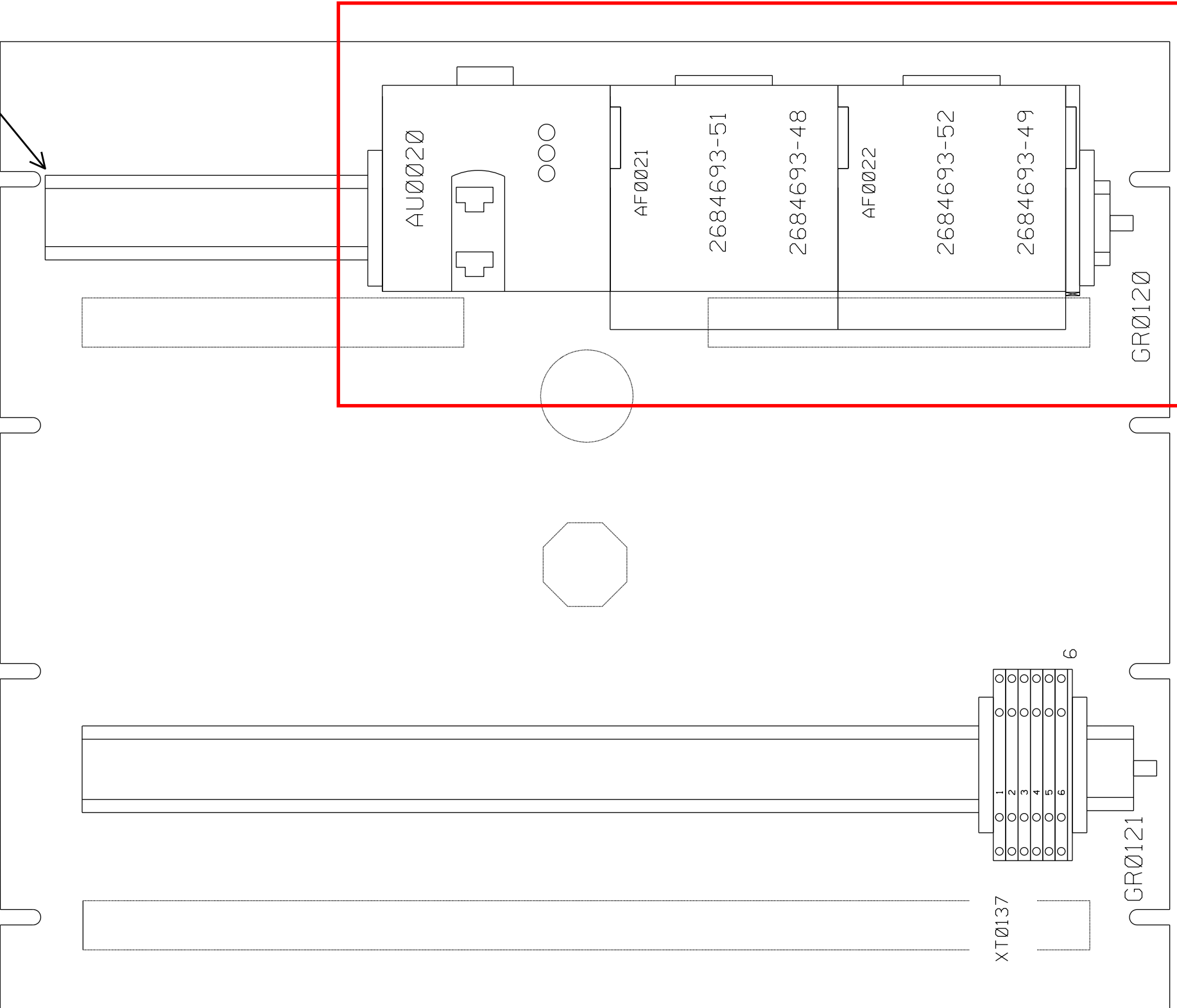
BACK VIEW WITH FLEX I/O INSTALLED
